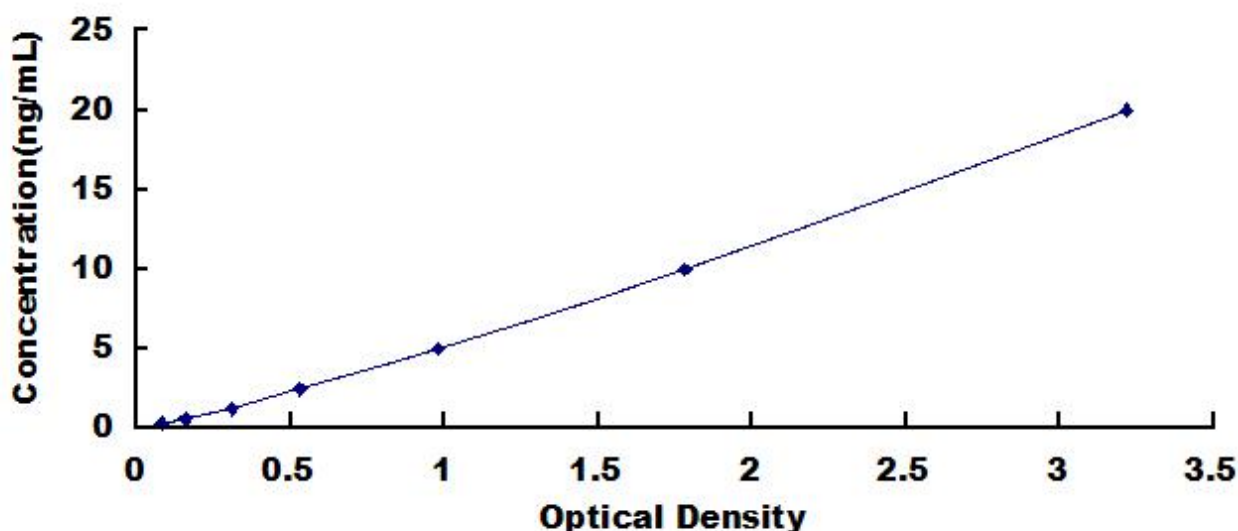
Typical Standard Curve for PI15, Human ELISA.
